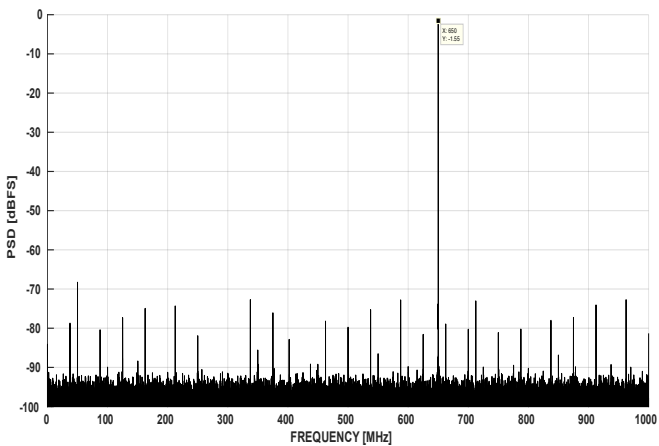
图 7-13. FFT at Fin = 650MHz, 2GSPS (1Vpp FS)
