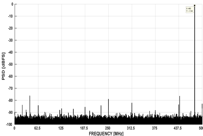
图 7-19. FFT at Fin = 400M Hz, 1GSPS (1Vpp FS)
