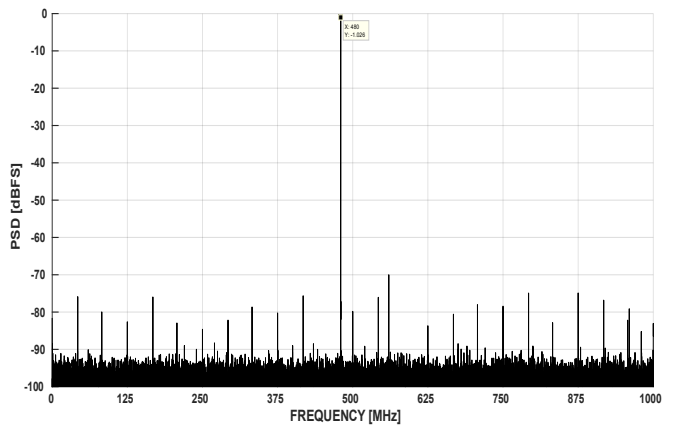
图 7-12. FFT at Fin = 480MHz, 2GSPS (1Vpp FS)
