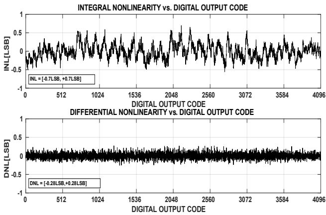
图 7-15. INL/DNL at Fin = 110MHz, 1GSPS (1Vpp FS)
