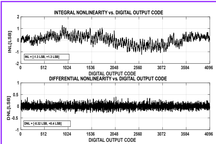
图 7-3. INL/DNL at Fin = 180MHz , 4GSPS (0.8Vpp FS)
