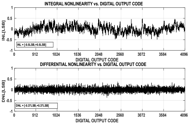
图 7-9. INL/DNL at Fin = 110MHz, 2GSPS (1Vpp FS)
