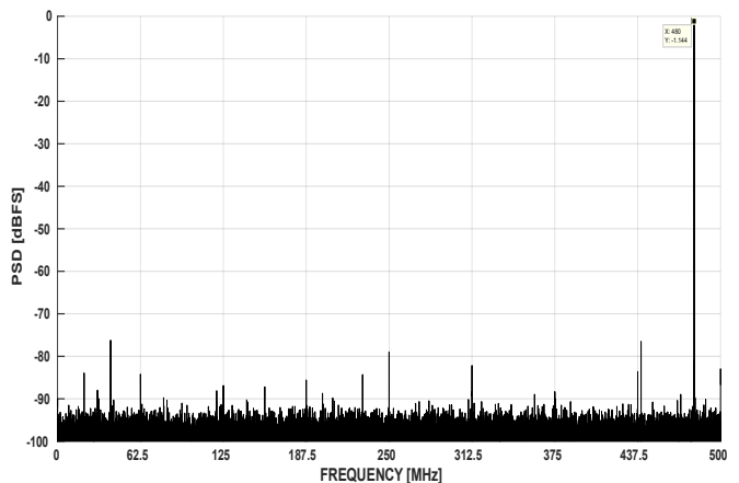
图 7-20. FFT at Fin = 480M Hz, 1GSPS (1Vpp FS)
